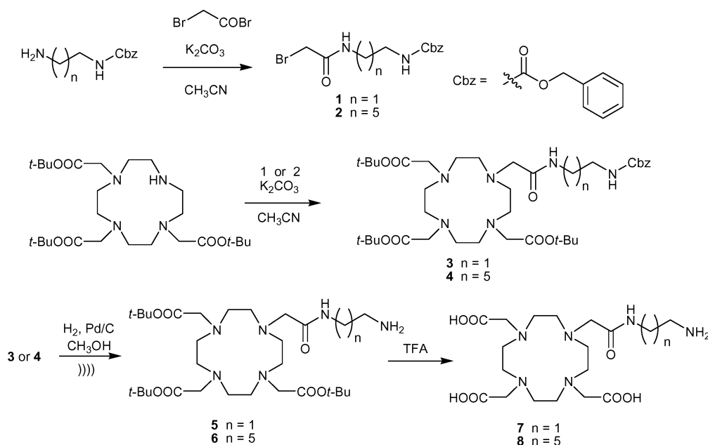
Scheme 2 Synthesis of DOTAMA( t -BuO) 3 en ( 5 ), DOTAMA( t -BuO) 3 C 6 NH 2 ( 6 ), DOTAMAen ( 7 ), DOTAMAC 6 NH 2 ( 8 )
