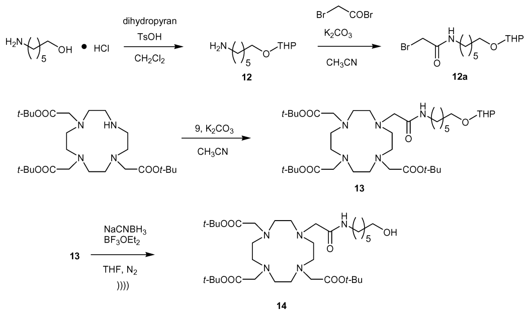
Scheme 4 Synthesis of bifunctional agent 14 .
