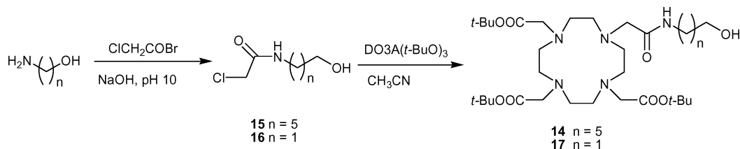
Scheme 5 Synthesis of bifunctional agents 14 and 17 without OH protection.
