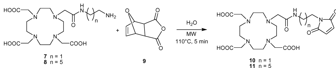
Scheme 3 Microwave-assisted synthesis of DOTA-monoamide maleimido derivatives.
