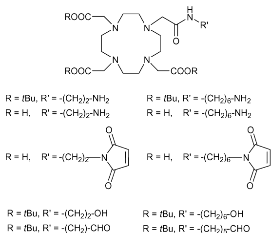
Scheme 1 DOTA-monoamide derivatives bearing different functional groups.
