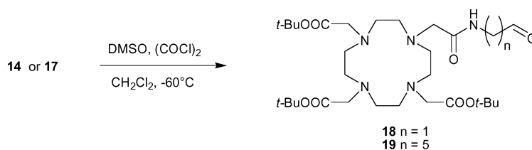
Scheme 6 Swern oxidation of 14 and 17 to yield aldehyde-containing DOTA-monoamide bifunctional agents 18 and 19 .
